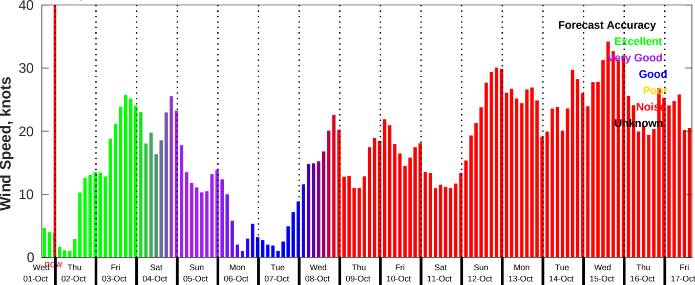
GFS Wind Speed Forecast for NDBC 46028 from 01-Oct-2025 16:00:00 to 17-Oct-2025 16:00:00
