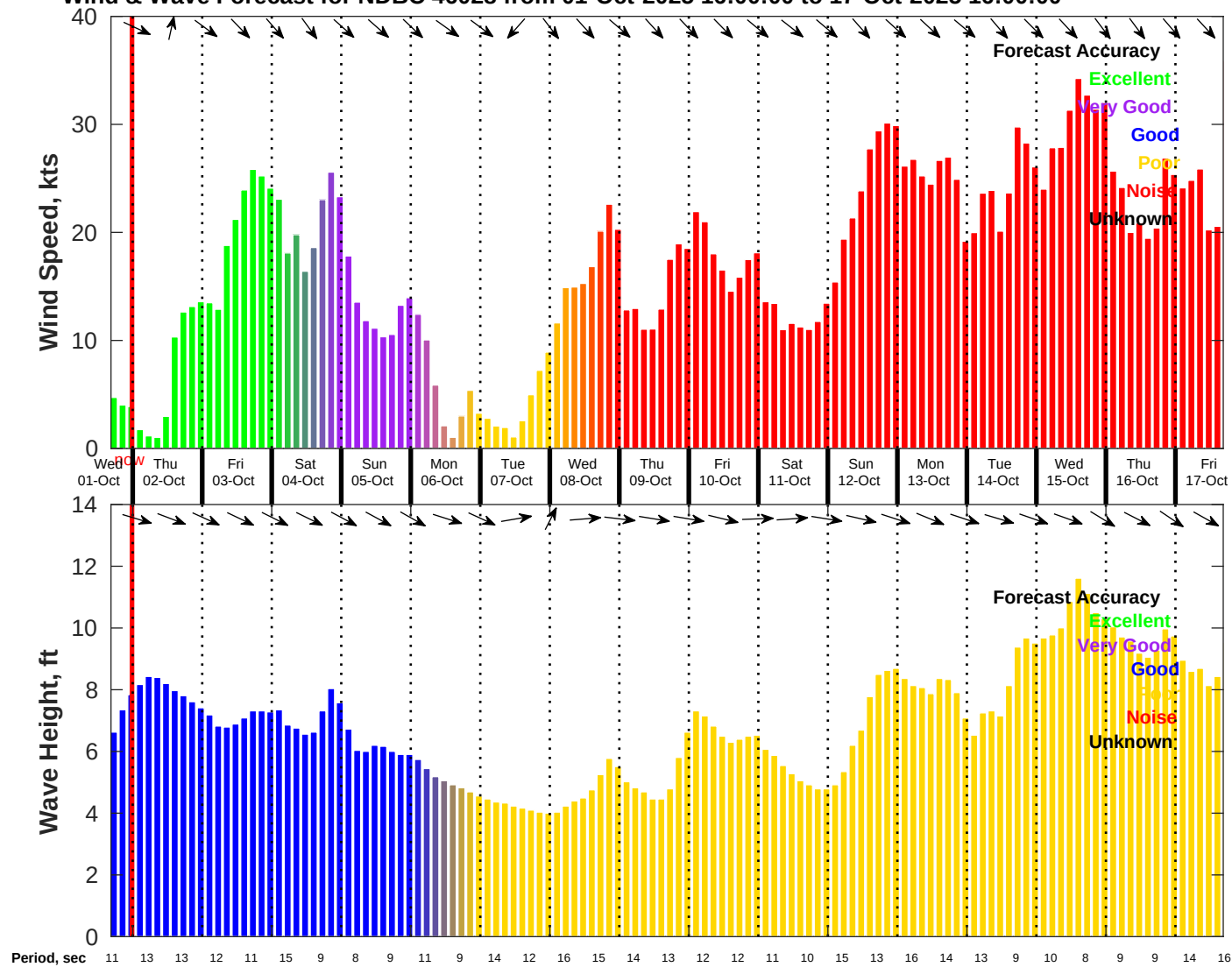
Wind & Wave Forecast for NDBC 46028 from 01-Oct-2025 16:00:00 to 17-Oct-2025 16:00:00
