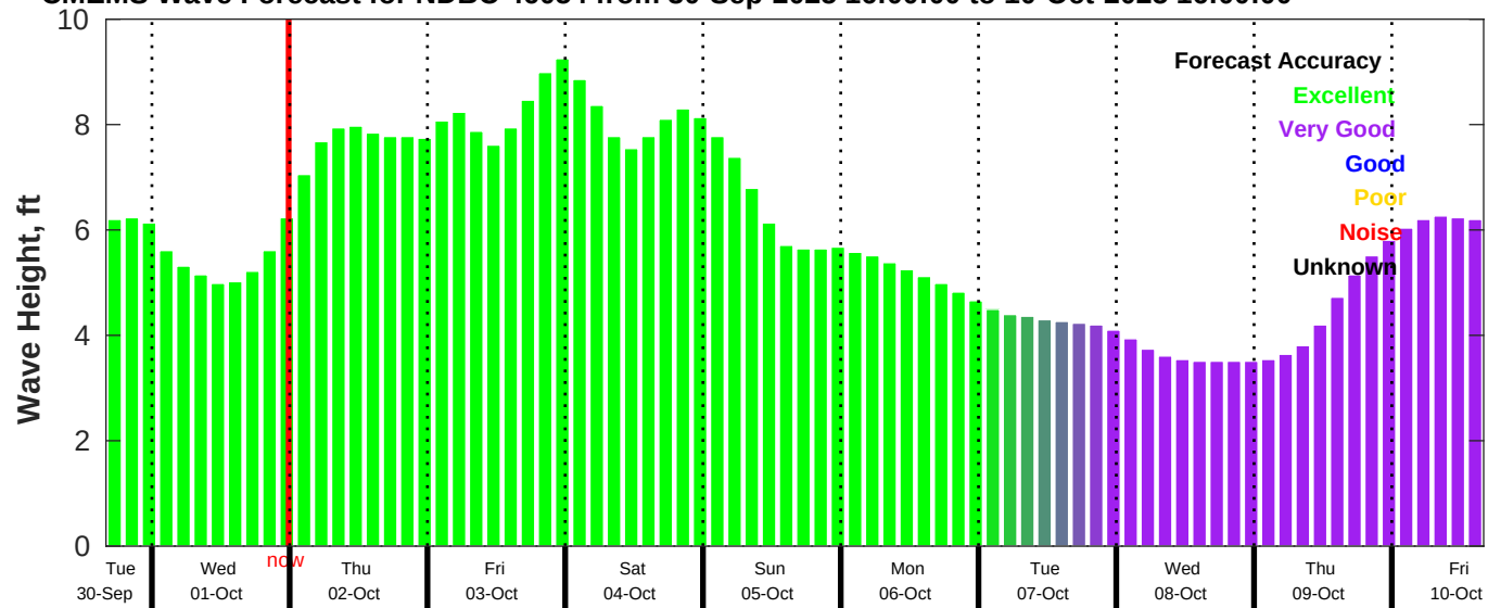
CMEMS Wave Forecast for NDBC 46054 from 30-Sep-2025 16:00:00 to 10-Oct-2025 16:00:00
