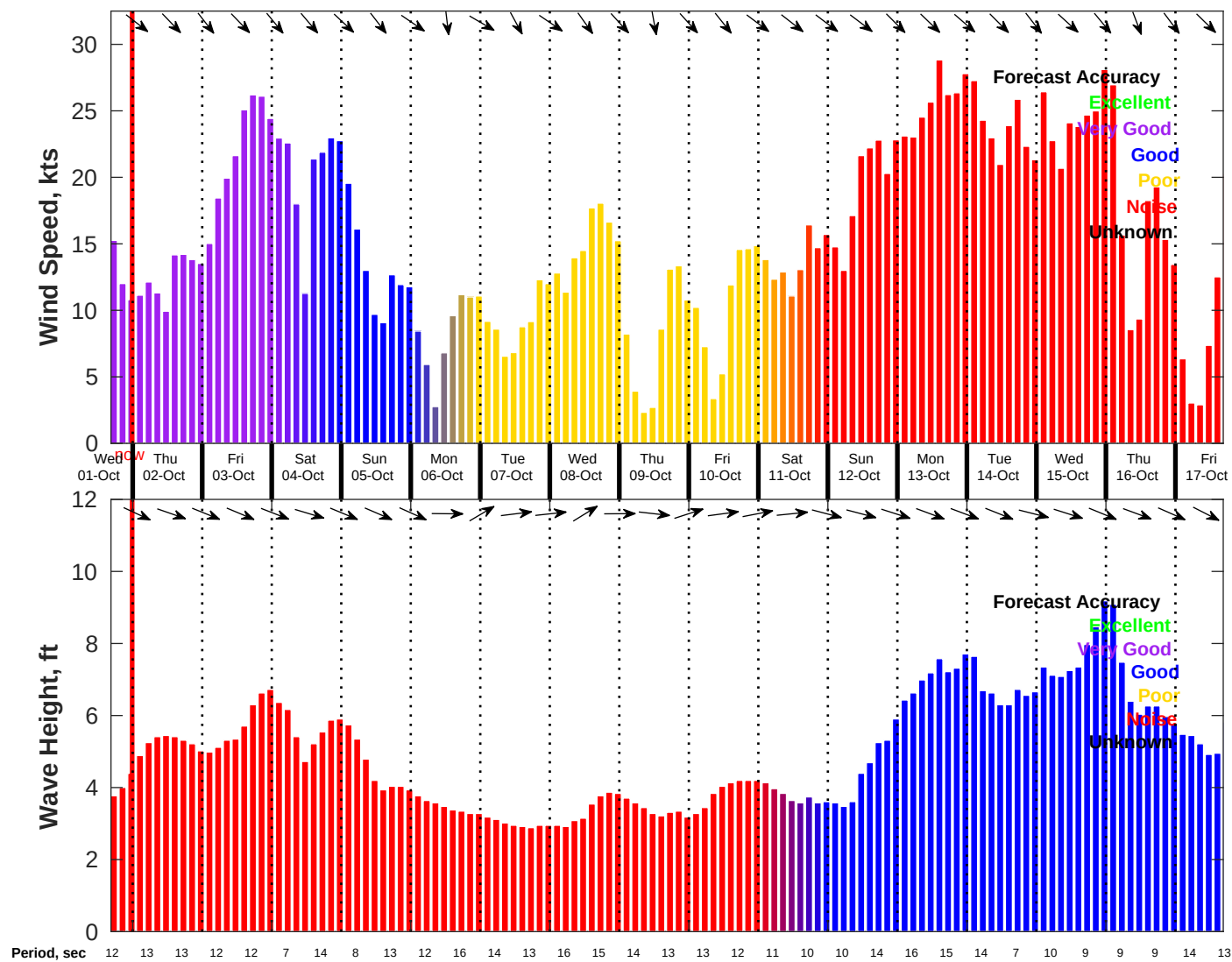
Wind & Wave Forecast for NDBC 46054 from 01-Oct-2025 16:00:00 to 17-Oct-2025 16:00:00
