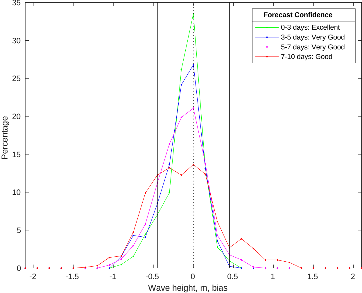
NDBC 46069 vs CMEMS Waves Bias Histogram: 02-Oct-2025
