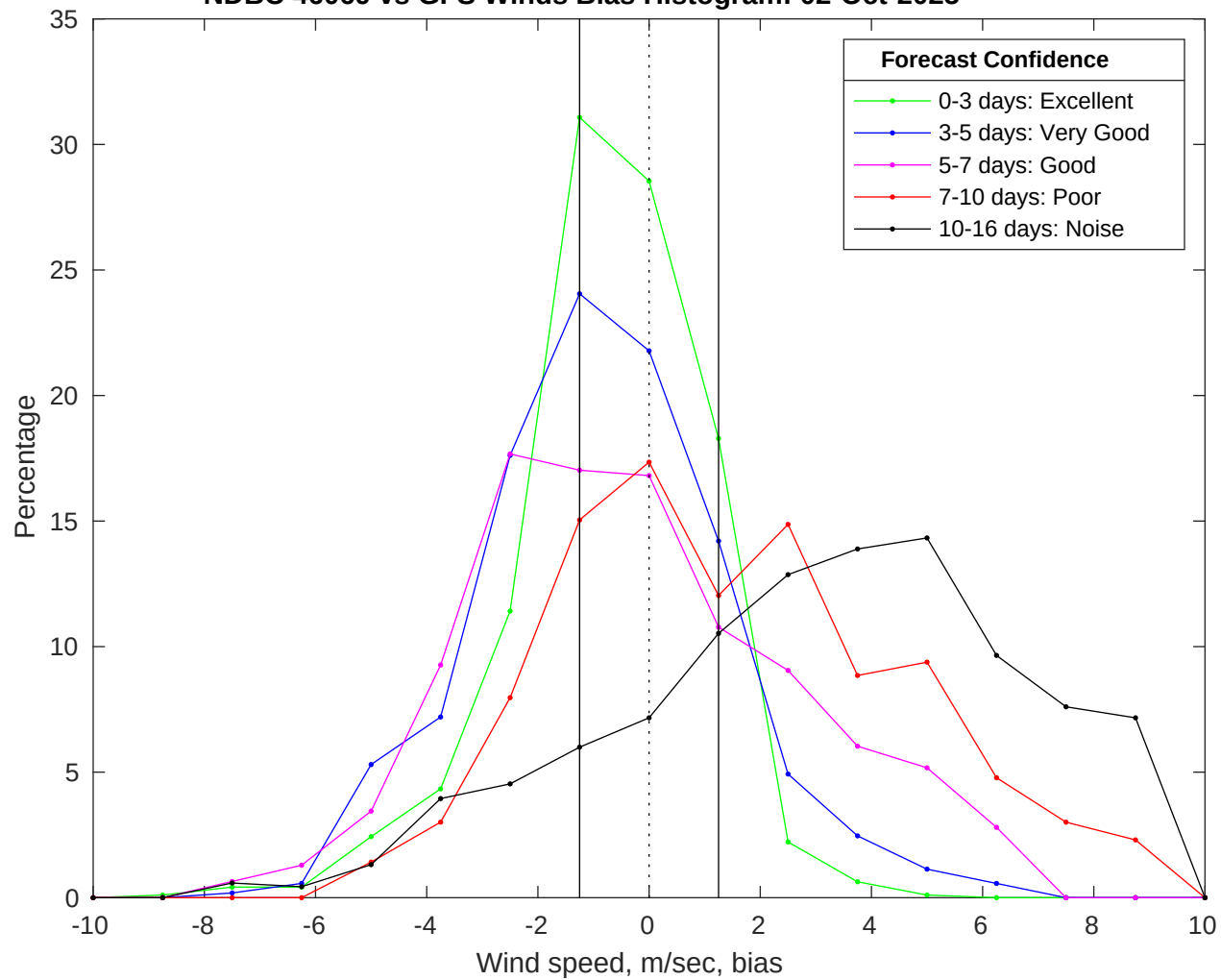
NDBC 46069 vs GFS Winds Bias Histogram: 02-Oct-2025
