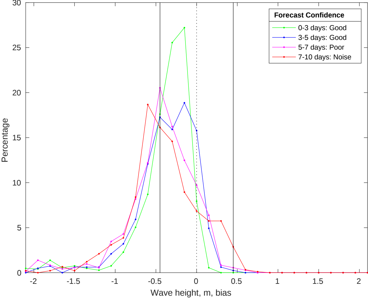
NDBC 51209 vs CMEMS Waves Bias Histogram: 02-Oct-2025
