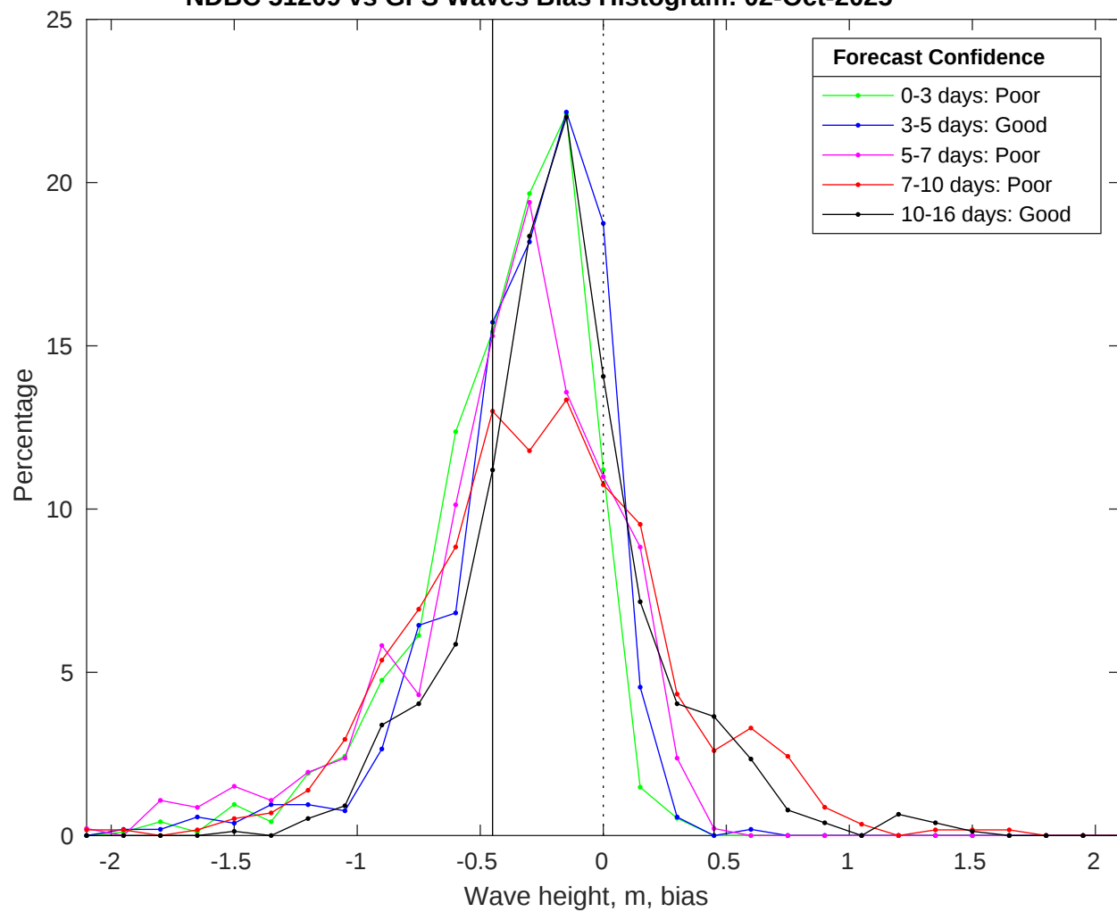
NDBC 51209 vs GFS Waves Bias Histogram: 02-Oct-2025
