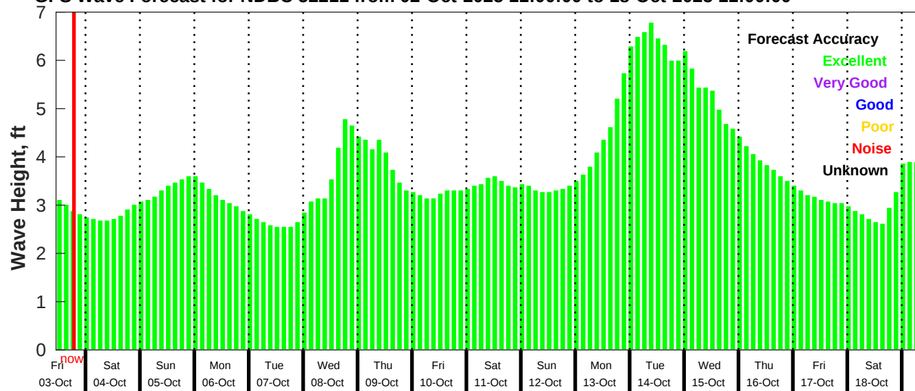
GFS Wave Forecast for NDBC 52211 from 02-Oct-2025 11:00:00 to 18-Oct-2025 11:00:00
