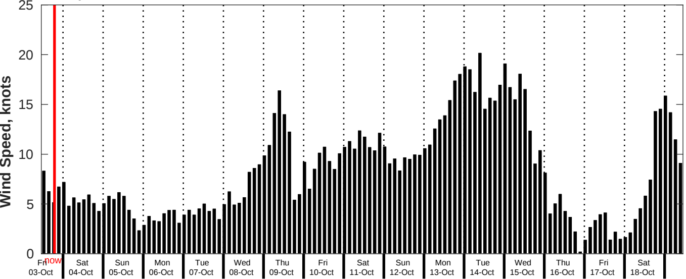
GFS Wind Speed Forecast for NDBC 52211 from 02-Oct-2025 11:00:00 to 18-Oct-2025 11:00:00
