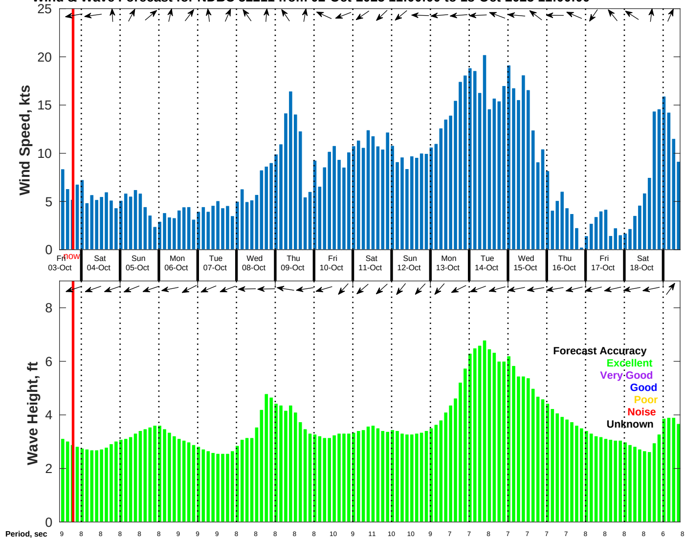
Wind & Wave Forecast for NDBC 52211 from 02-Oct-2025 11:00:00 to 18-Oct-2025 11:00:00
