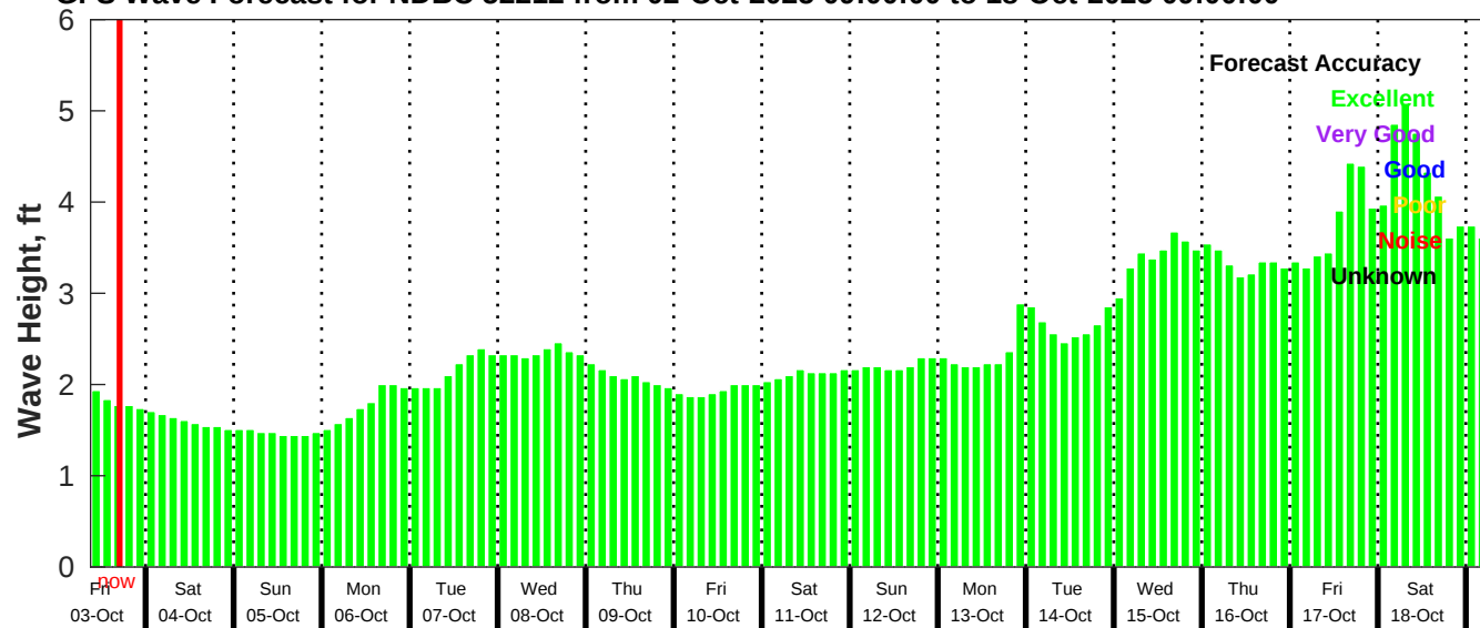
GFS Wave Forecast for NDBC 52212 from 02-Oct-2025 09:00:00 to 18-Oct-2025 09:00:00
