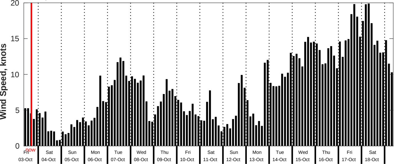
GFS Wind Speed Forecast for NDBC 52212 from 02-Oct-2025 09:00:00 to 18-Oct-2025 09:00:00
