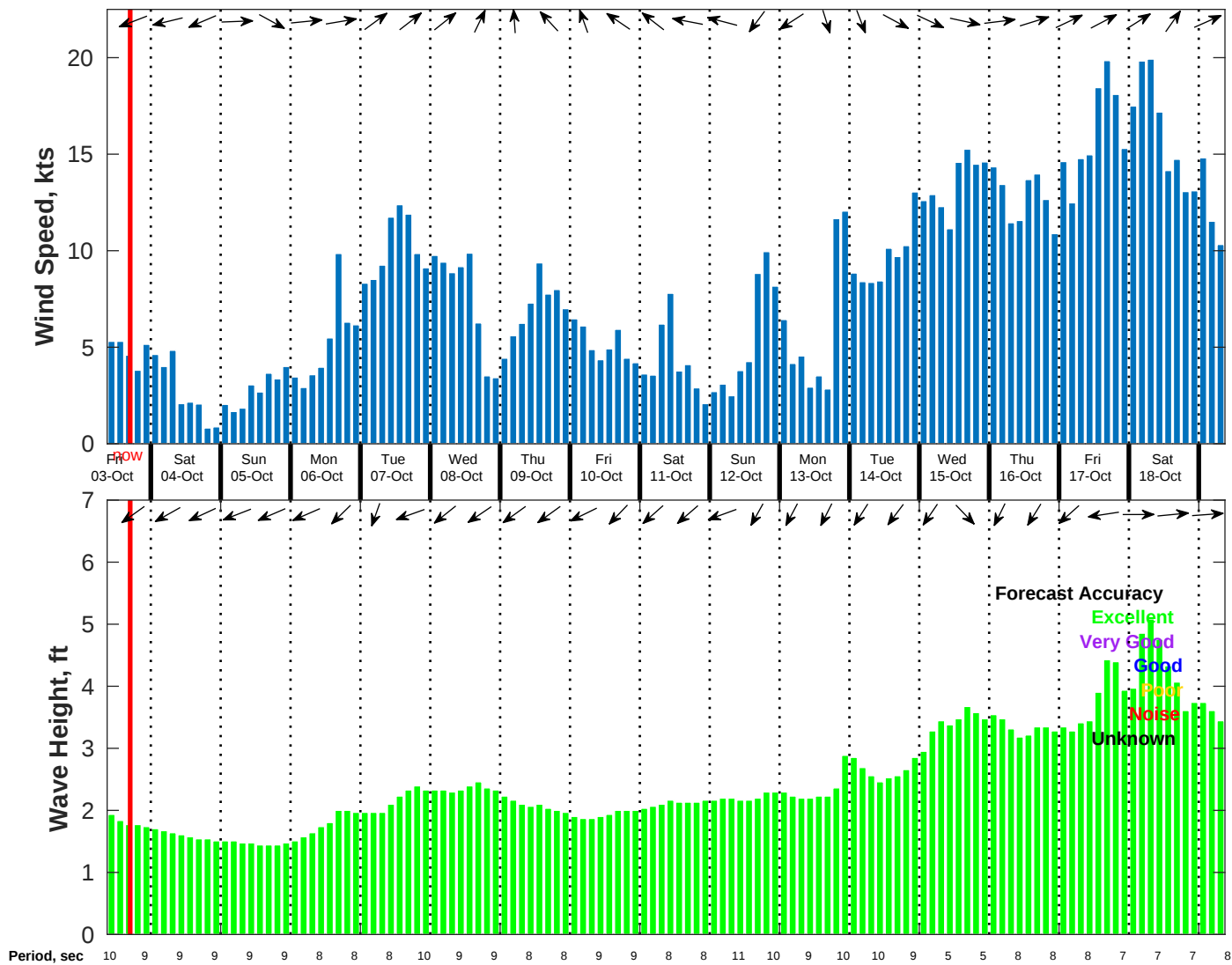
Wind & Wave Forecast for NDBC 52212 from 02-Oct-2025 09:00:00 to 18-Oct-2025 09:00:00
