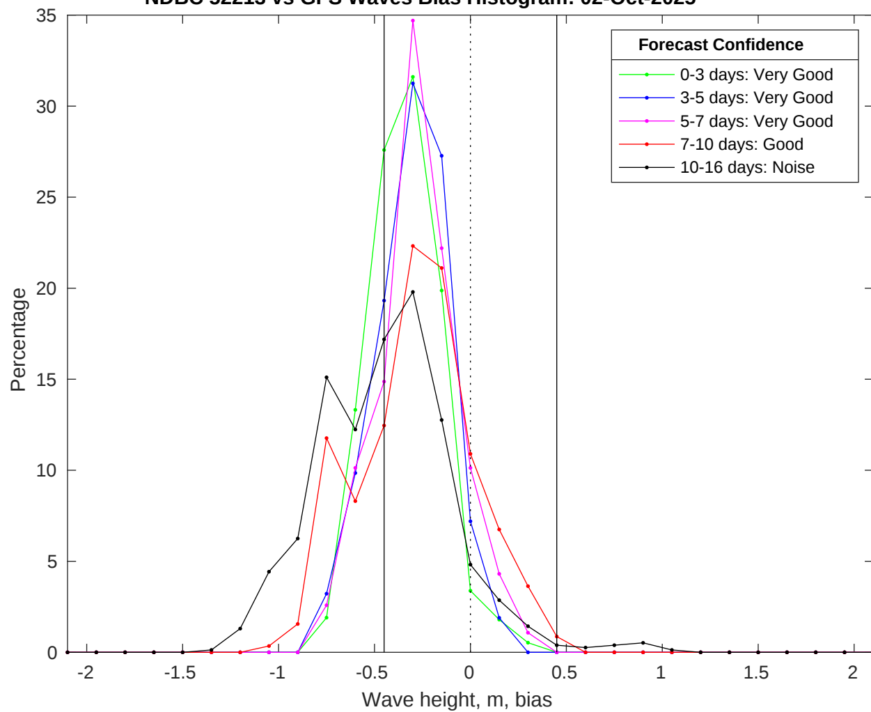
NDBC 52213 vs GFS Waves Bias Histogram: 02-Oct-2025
