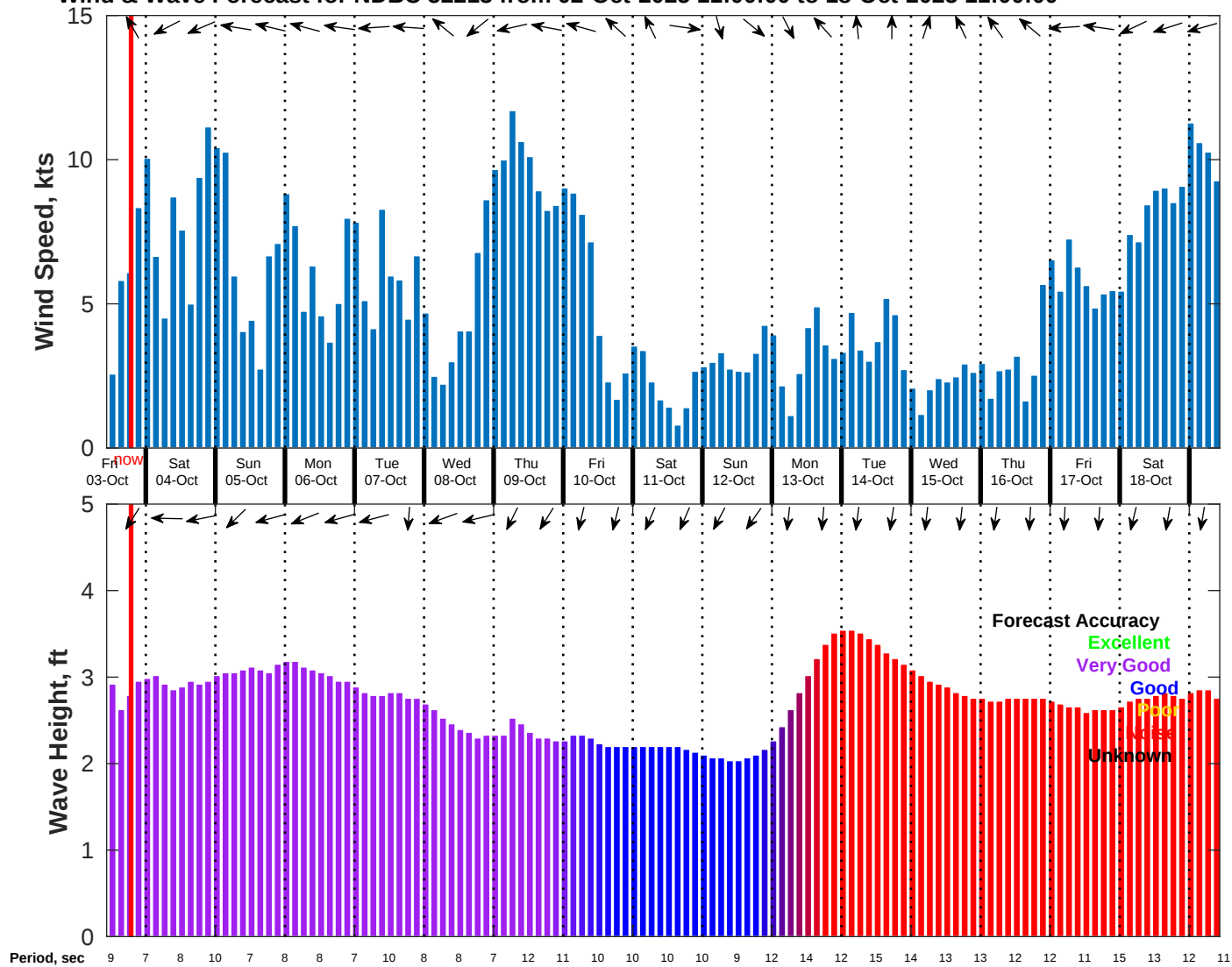
Wind & Wave Forecast for NDBC 52213 from 02-Oct-2025 11:00:00 to 18-Oct-2025 11:00:00
