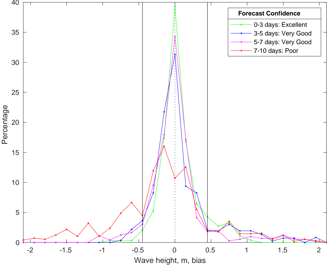
NDBC 41004 vs CMEMS Waves Bias Histogram: 03-Oct-2025
