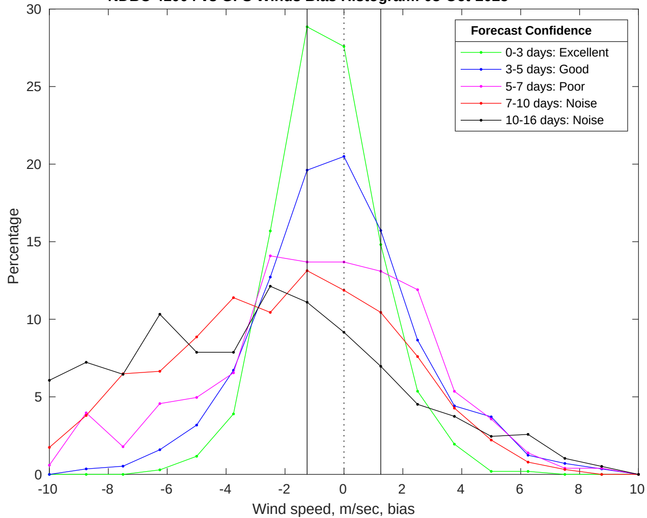
NDBC 41004 vs GFS Winds Bias Histogram: 03-Oct-2025
