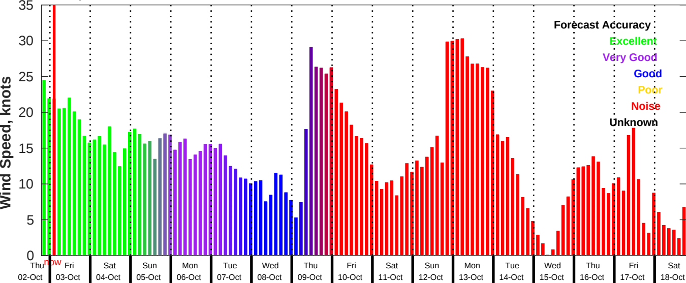
GFS Wind Speed Forecast for NDBC 41013 from 02-Oct-2025 19:00:00 to 18-Oct-2025 19:00:00
