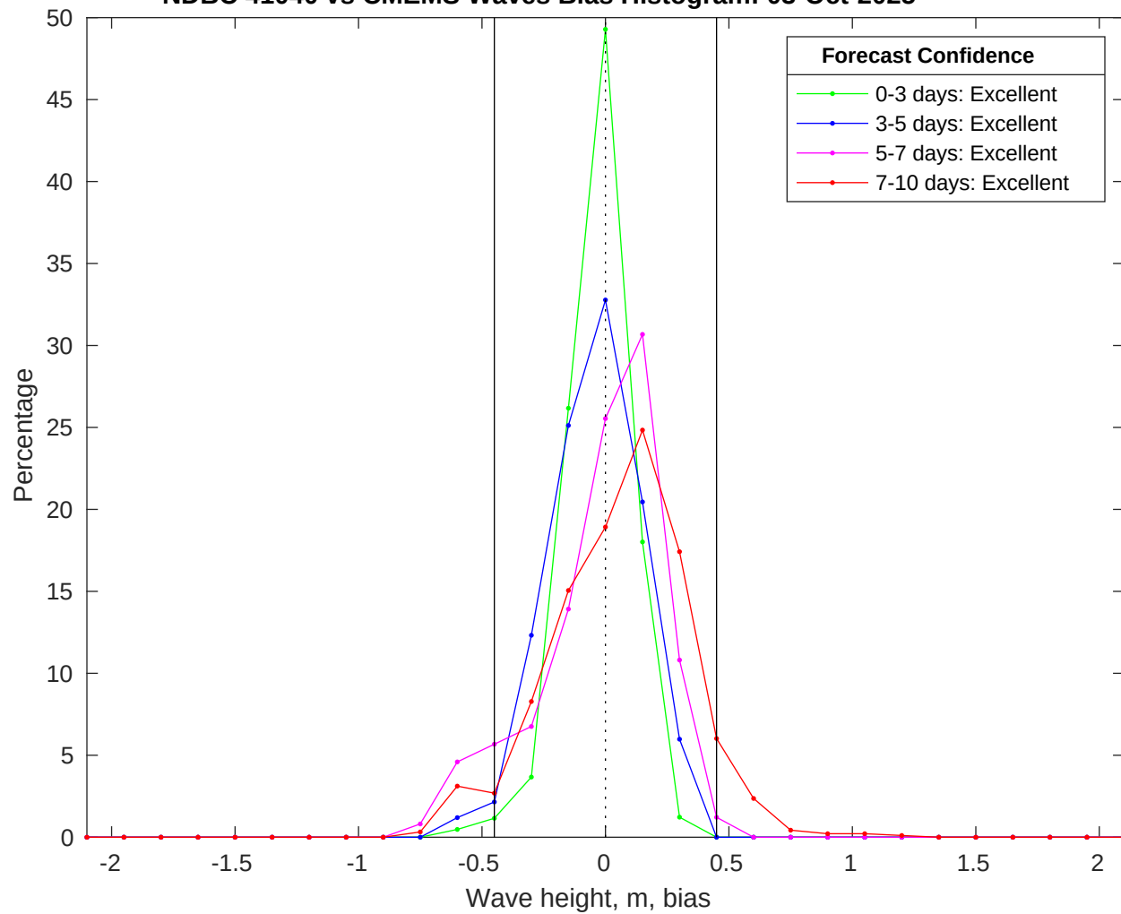
NDBC 41040 vs CMEMS Waves Bias Histogram: 03-Oct-2025
