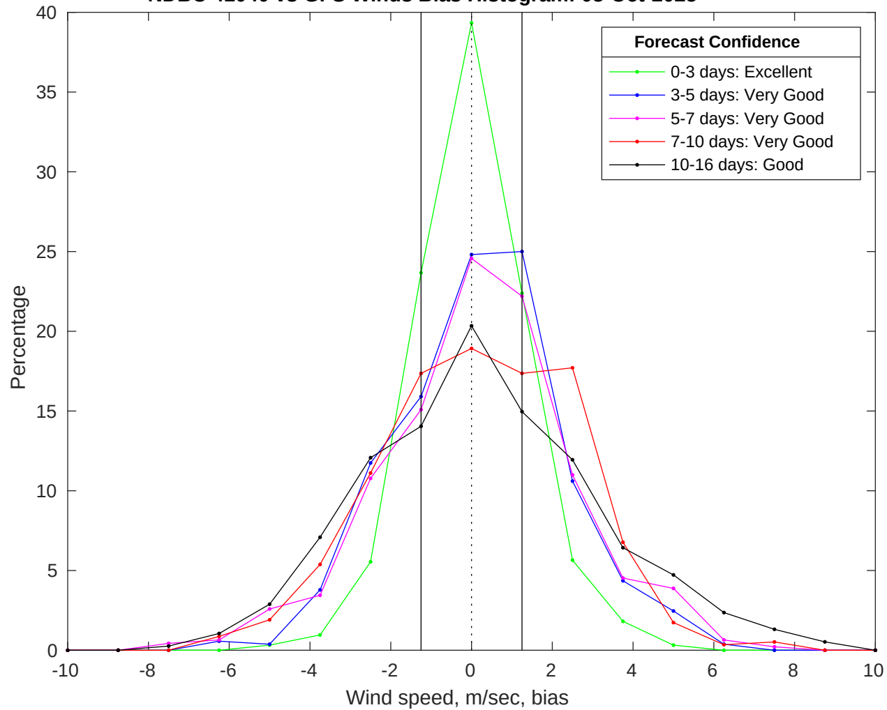
NDBC 41040 vs GFS Winds Bias Histogram: 03-Oct-2025
