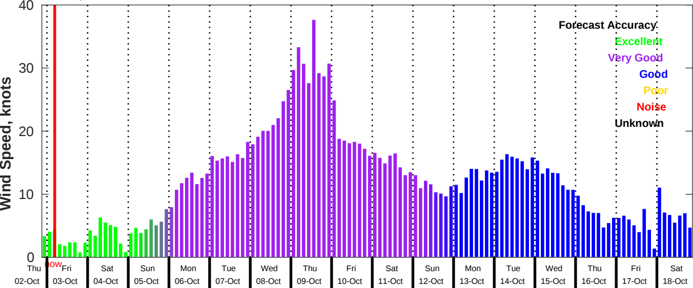
GFS Wind Speed Forecast for NDBC 41040 from 02-Oct-2025 21:00:00 to 18-Oct-2025 21:00:00
