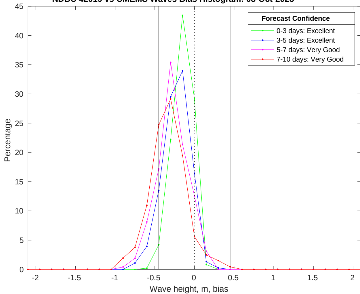
NDBC 42019 vs CMEMS Waves Bias Histogram: 03-Oct-2025
