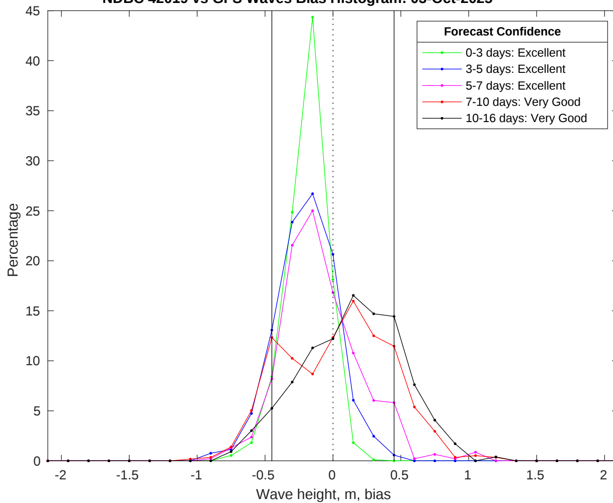
NDBC 42019 vs GFS Waves Bias Histogram: 03-Oct-2025
