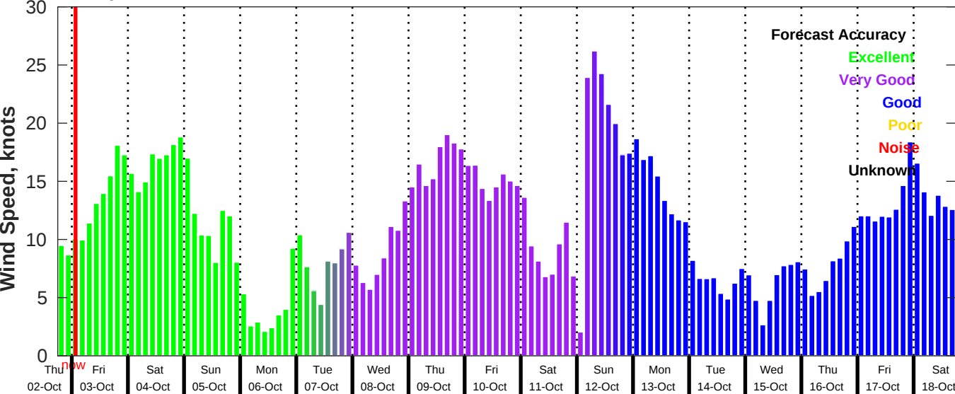
GFS Wind Speed Forecast for NDBC 42019 from 02-Oct-2025 18:00:00 to 18-Oct-2025 18:00:00
