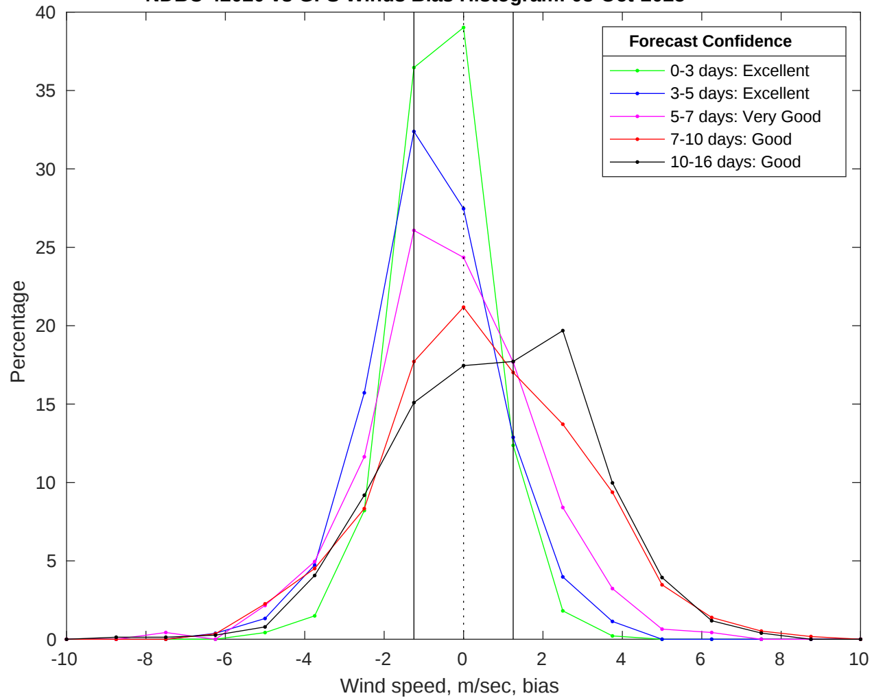
NDBC 42020 vs GFS Winds Bias Histogram: 03-Oct-2025
