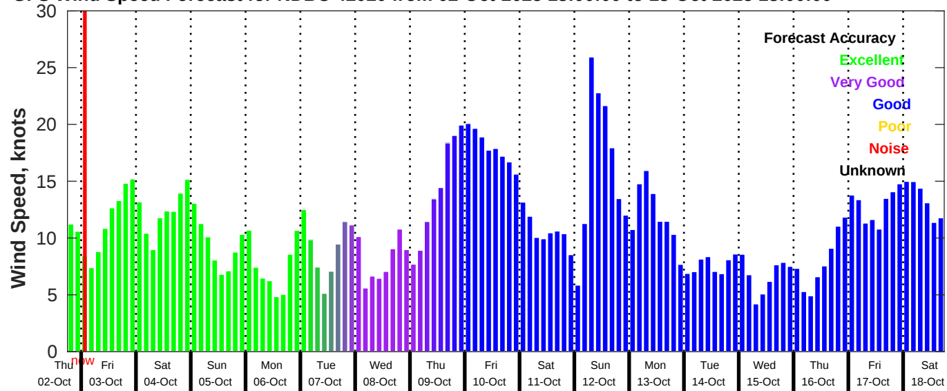
GFS Wind Speed Forecast for NDBC 42020 from 02-Oct-2025 18:00:00 to 18-Oct-2025 18:00:00
