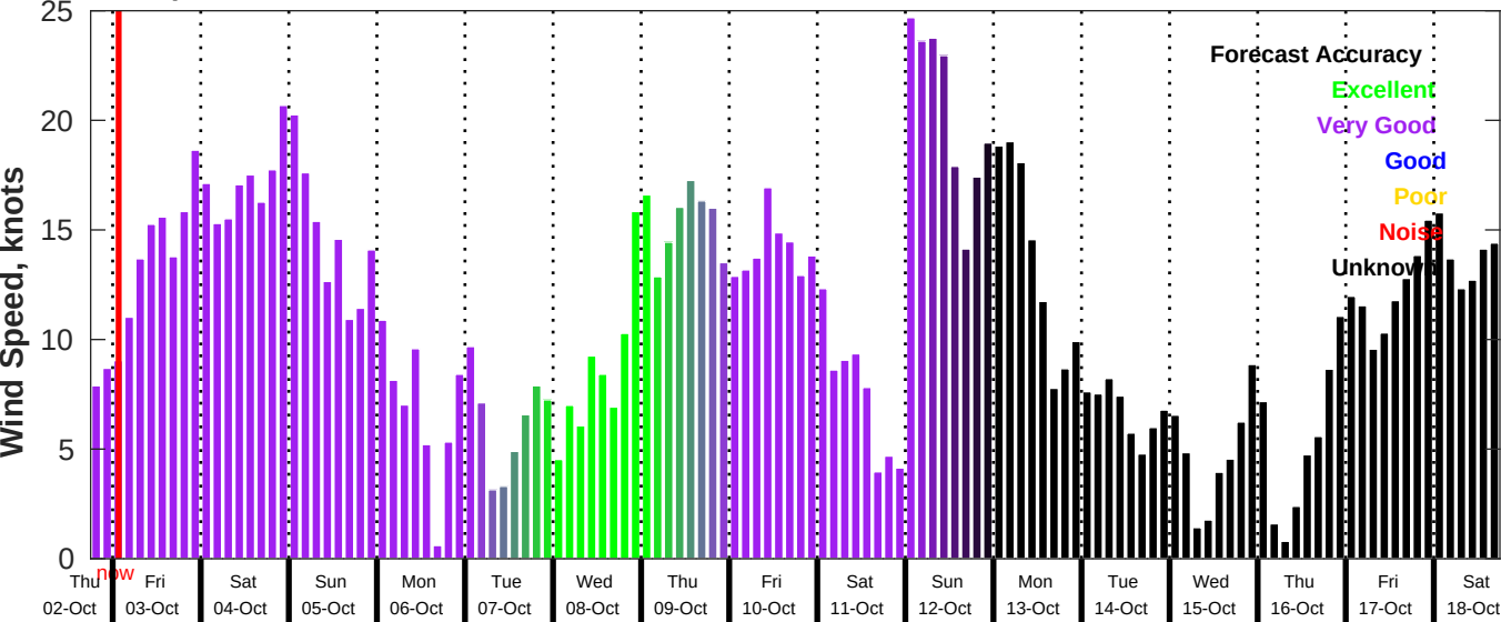
GFS Wind Speed Forecast for NDBC 42035 from 02-Oct-2025 18:00:00 to 18-Oct-2025 18:00:00
