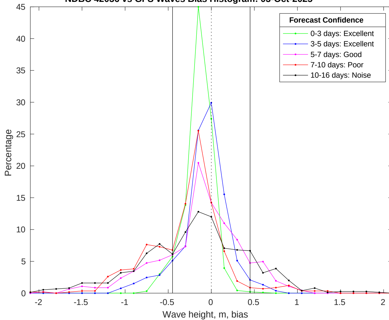
NDBC 42036 vs GFS Waves Bias Histogram: 03-Oct-2025
