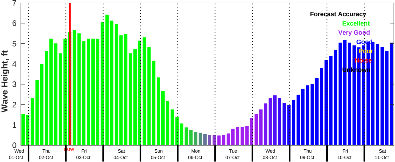
CMEMS Wave Forecast for NDBC 42036 from 01-Oct-2025 19:00:00 to 11-Oct-2025 19:00:00
