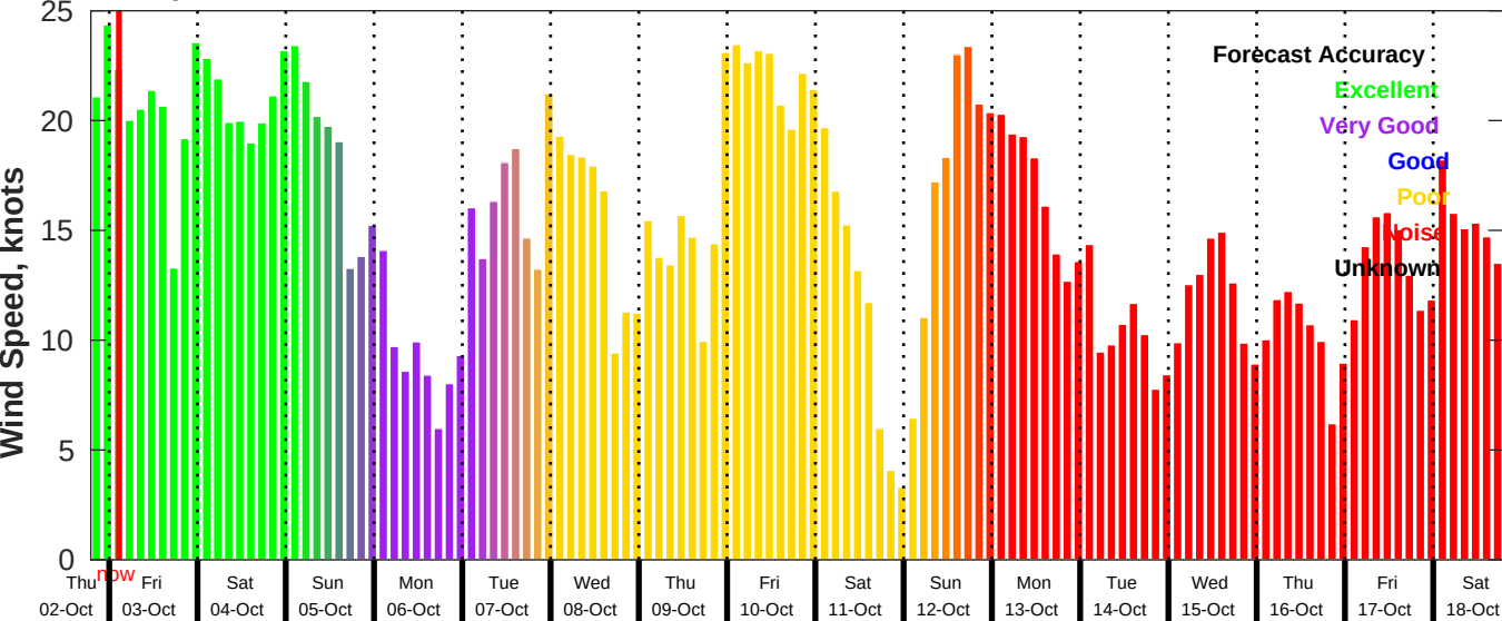
GFS Wind Speed Forecast for NDBC 42036 from 02-Oct-2025 19:00:00 to 18-Oct-2025 19:00:00
