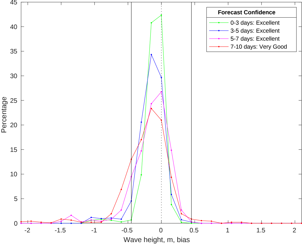
NDBC 42040 vs CMEMS Waves Bias Histogram: 03-Oct-2025
