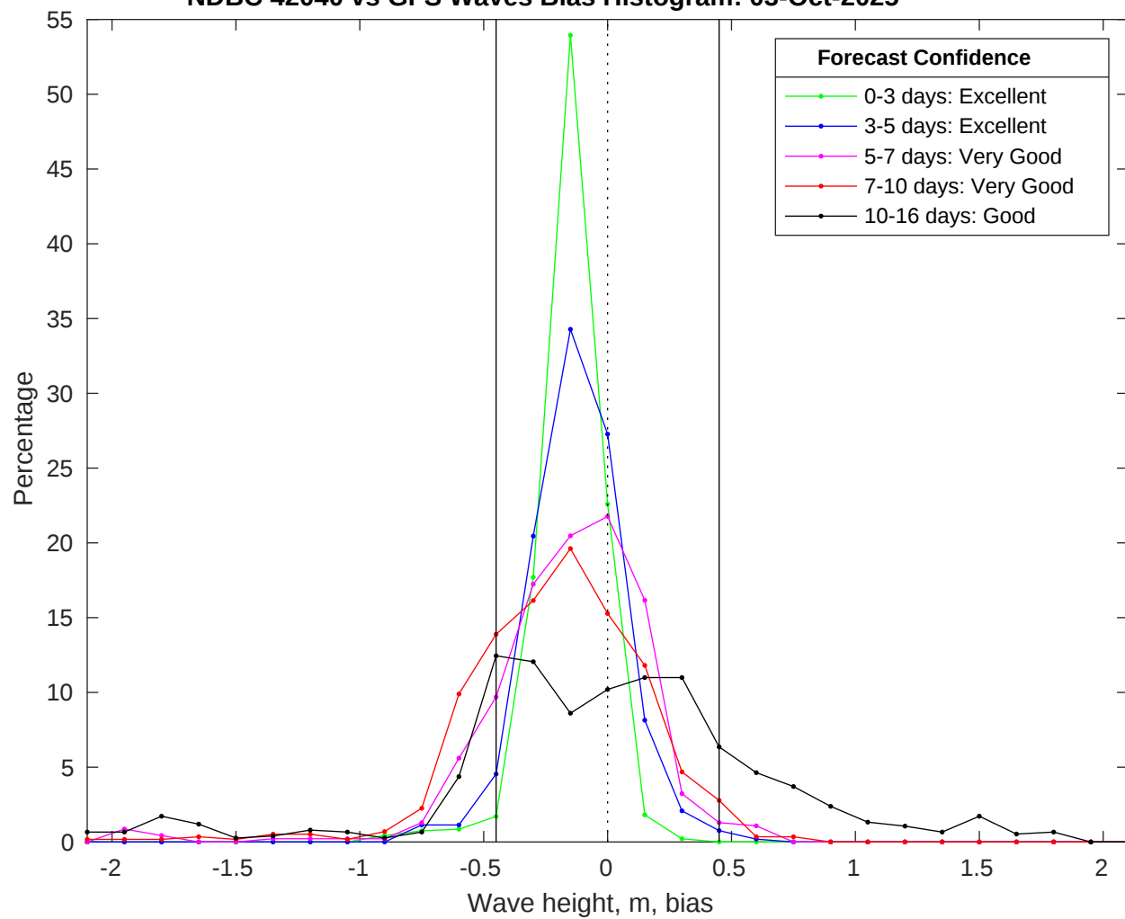
NDBC 42040 vs GFS Waves Bias Histogram: 03-Oct-2025
