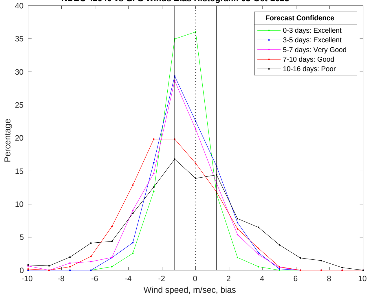
NDBC 42040 vs GFS Winds Bias Histogram: 03-Oct-2025
