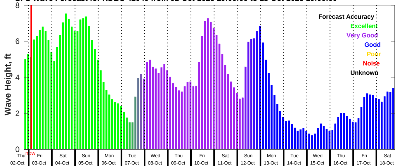
GFS Wave Forecast for NDBC 42040 from 02-Oct-2025 19:00:00 to 18-Oct-2025 19:00:00
