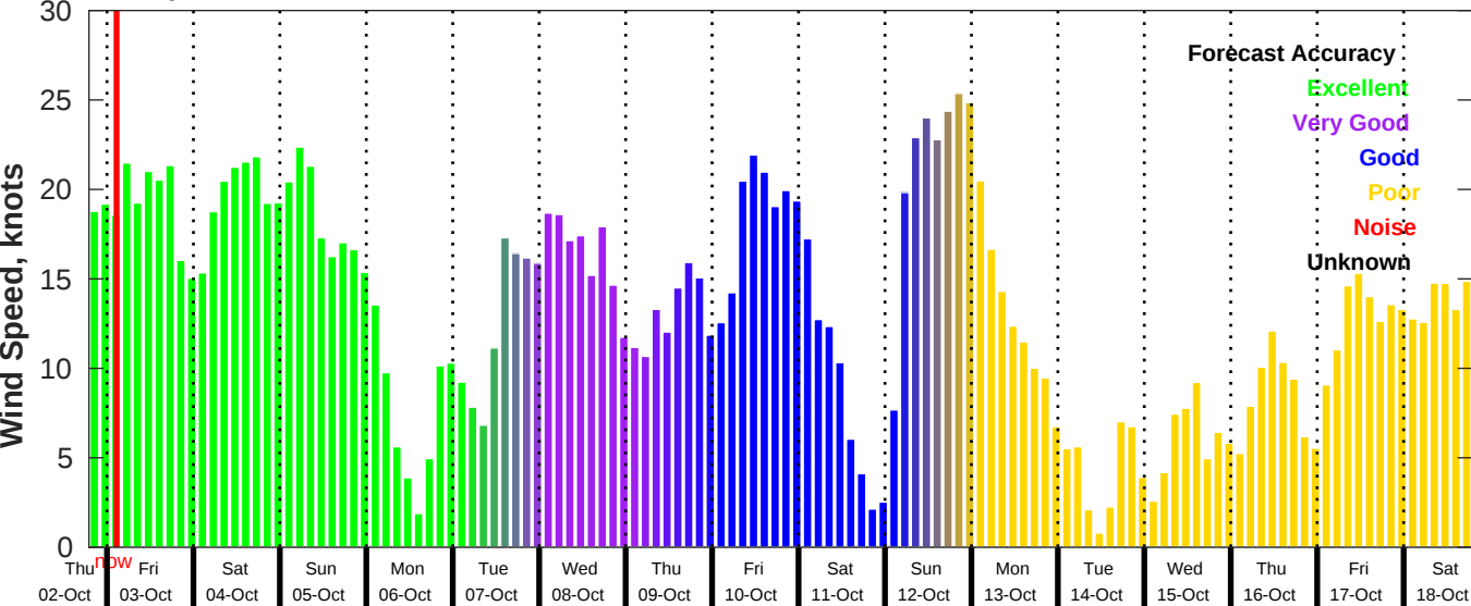
GFS Wind Speed Forecast for NDBC 42040 from 02-Oct-2025 19:00:00 to 18-Oct-2025 19:00:00
