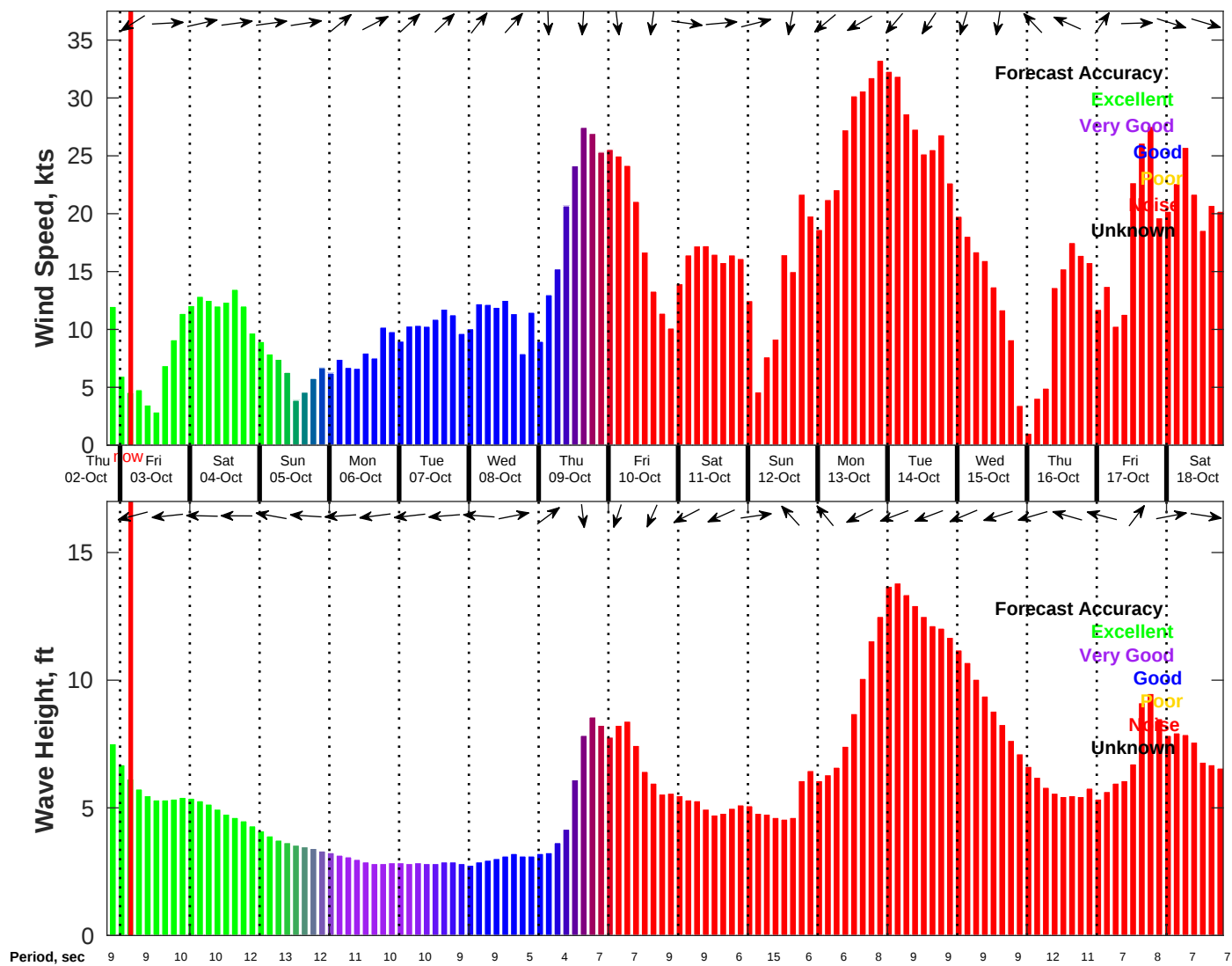
Wind & Wave Forecast for NDBC 44008 from 02-Oct-2025 20:00:00 to 18-Oct-2025 20:00:00
