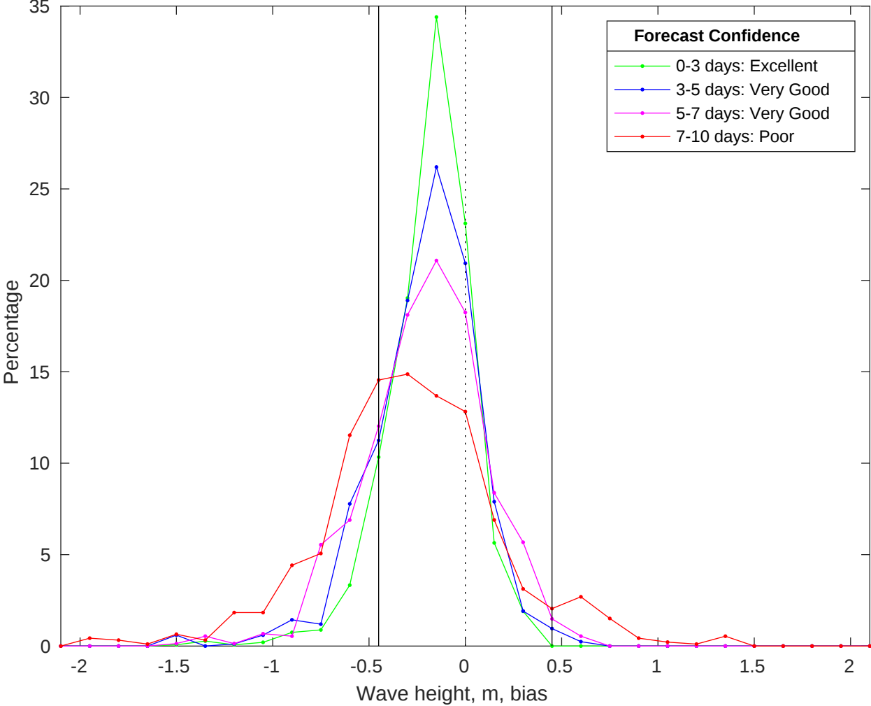
NDBC 46011 vs CMEMS Waves Bias Histogram: 03-Oct-2025
