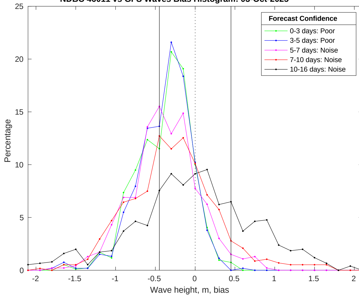
NDBC 46011 vs GFS Waves Bias Histogram: 03-Oct-2025
