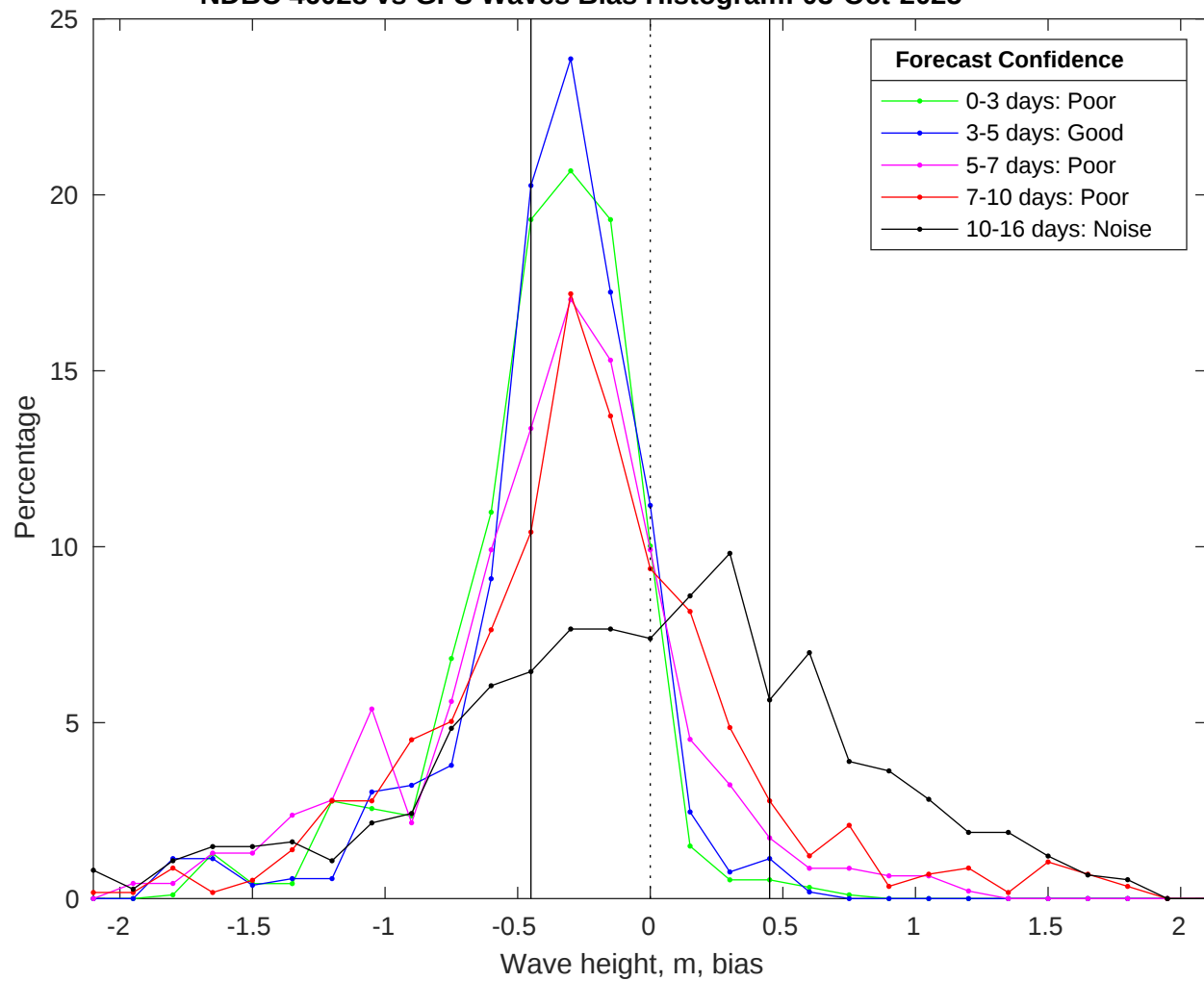
NDBC 46028 vs GFS Waves Bias Histogram: 03-Oct-2025
