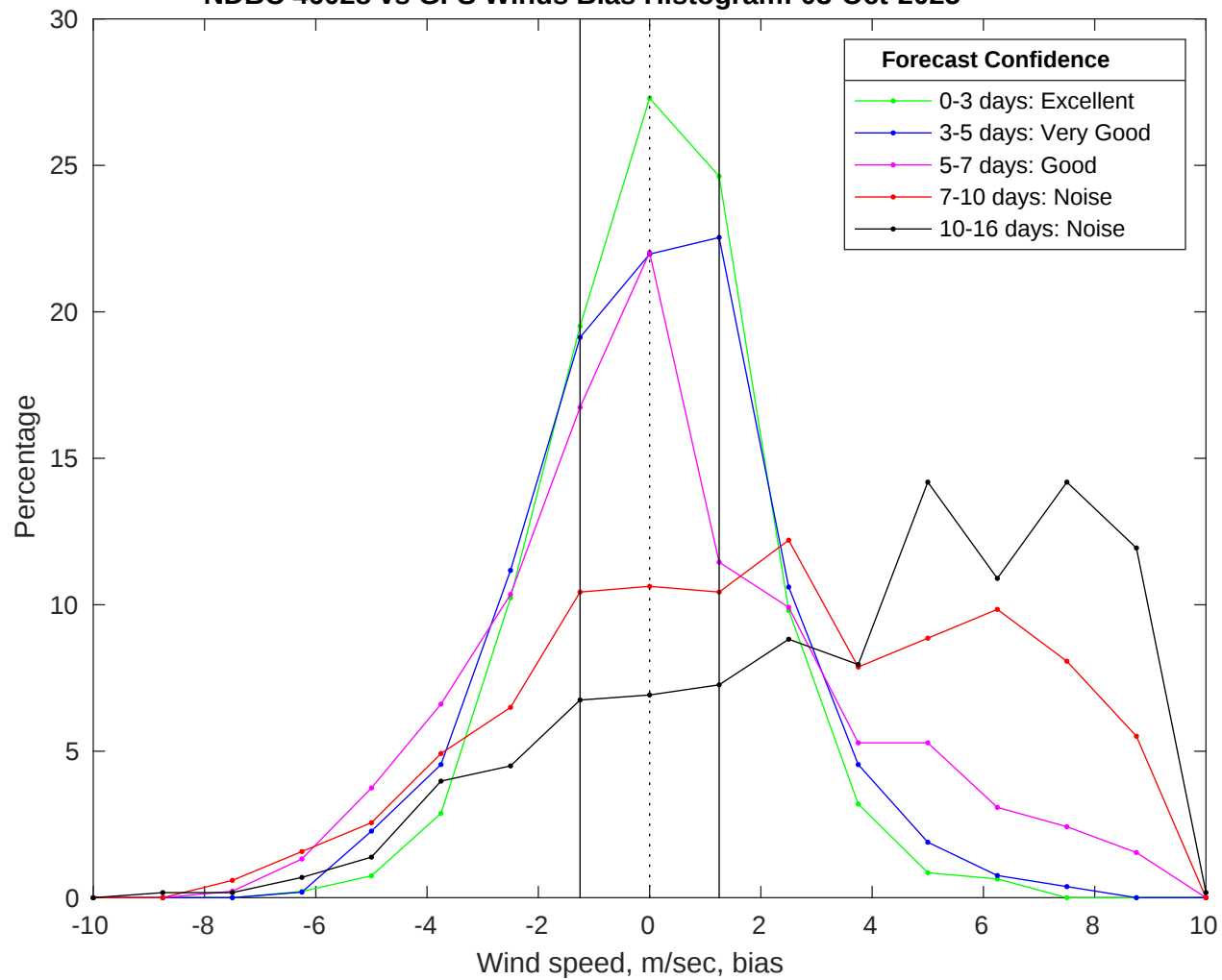
NDBC 46028 vs GFS Winds Bias Histogram: 03-Oct-2025
