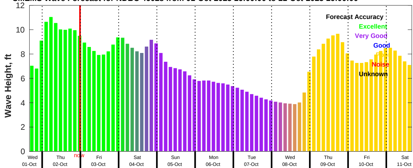
CMEMS Wave Forecast for NDBC 46028 from 01-Oct-2025 16:00:00 to 11-Oct-2025 16:00:00
