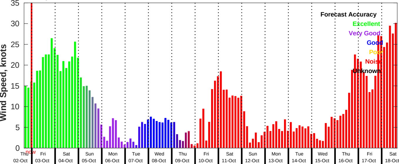
GFS Wind Speed Forecast for NDBC 46028 from 02-Oct-2025 16:00:00 to 18-Oct-2025 16:00:00
