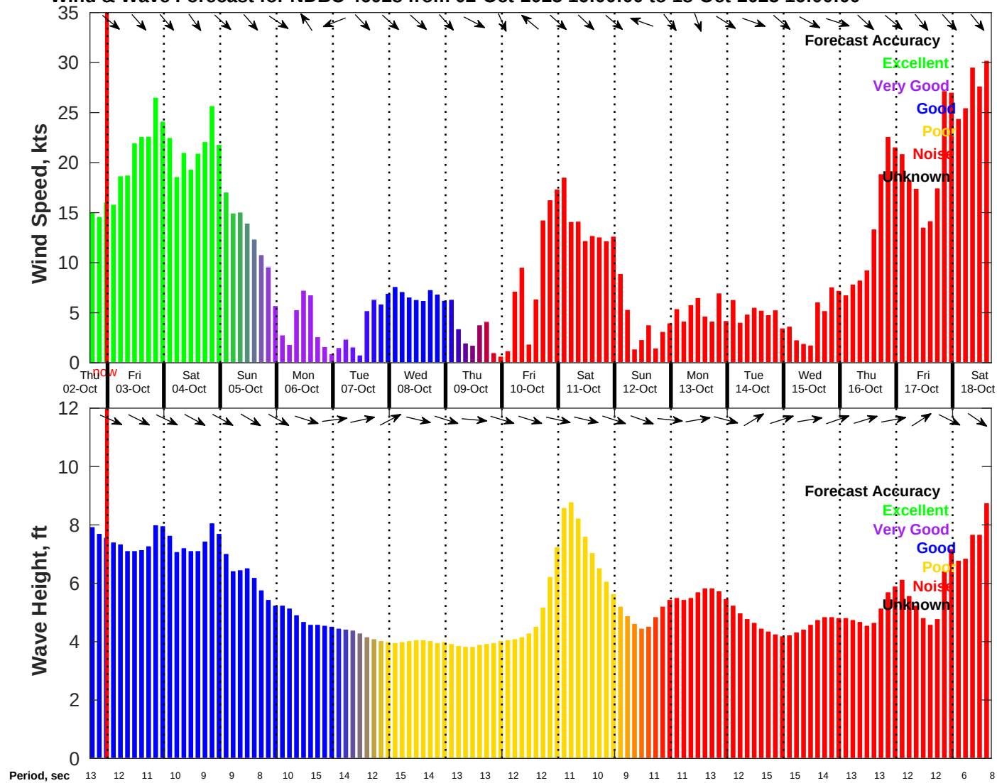
Wind & Wave Forecast for NDBC 46028 from 02-Oct-2025 16:00:00 to 18-Oct-2025 16:00:00
