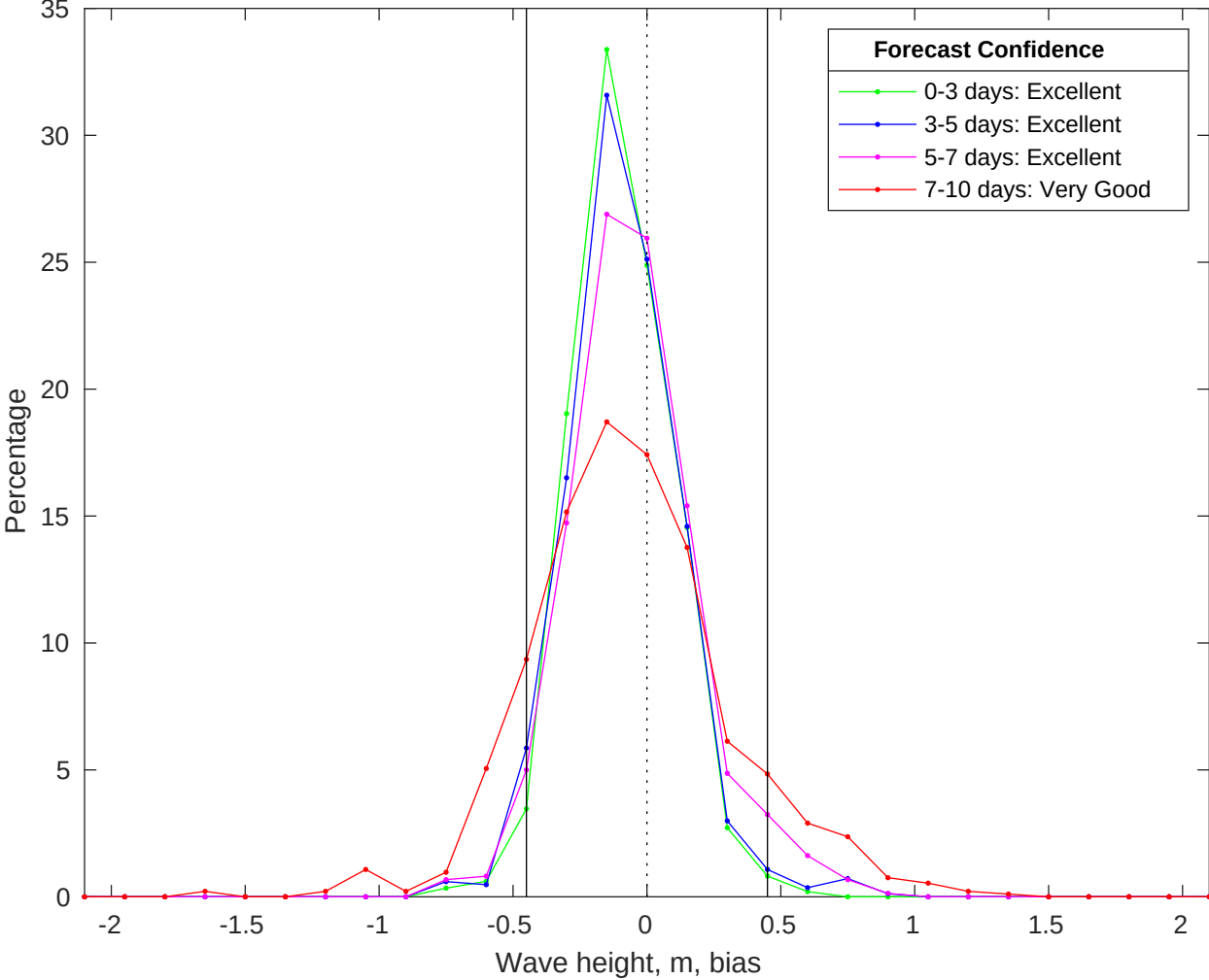
NDBC 46054 vs CMEMS Waves Bias Histogram: 03-Oct-2025
