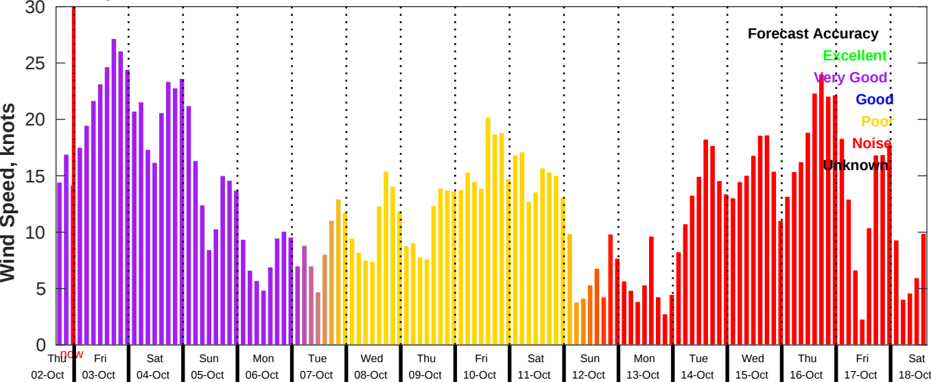
GFS Wind Speed Forecast for NDBC 46054 from 02-Oct-2025 16:00:00 to 18-Oct-2025 16:00:00
