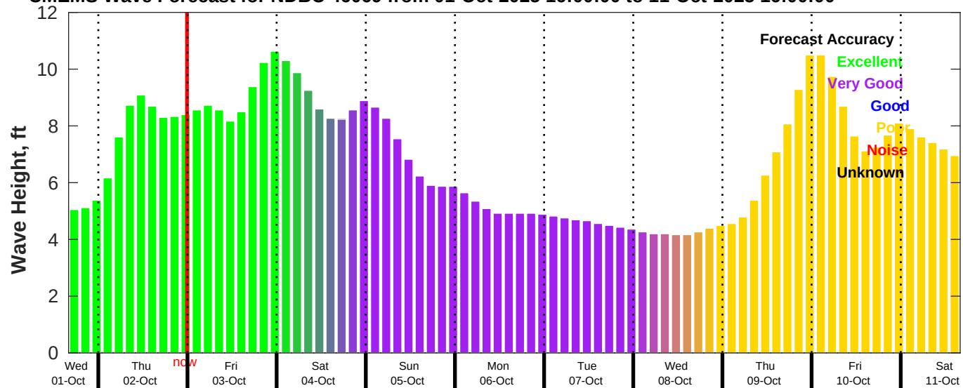
CMEMS Wave Forecast for NDBC 46069 from 01-Oct-2025 16:00:00 to 11-Oct-2025 16:00:00
