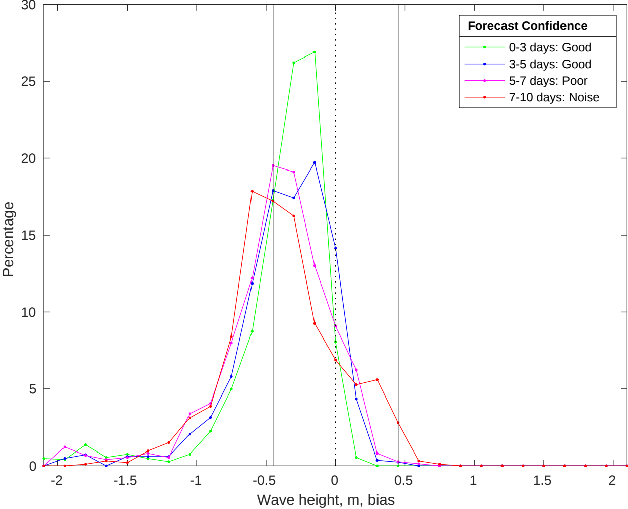
NDBC 51209 vs CMEMS Waves Bias Histogram: 03-Oct-2025
