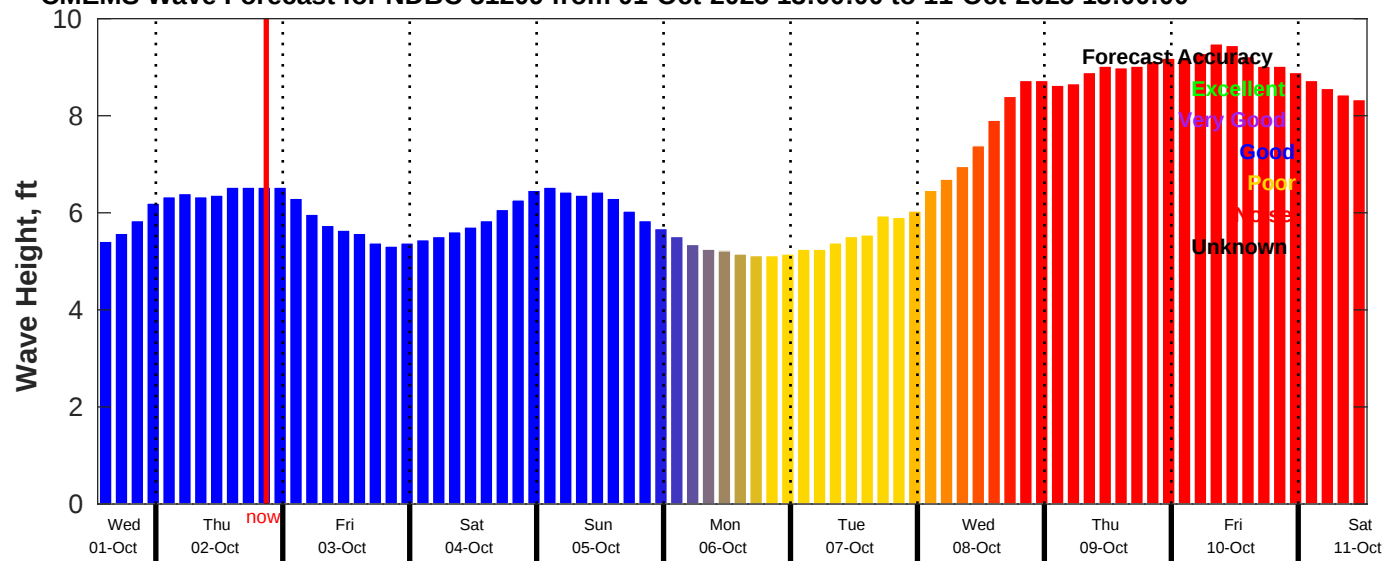
CMEMS Wave Forecast for NDBC 51209 from 01-Oct-2025 13:00:00 to 11-Oct-2025 13:00:00
