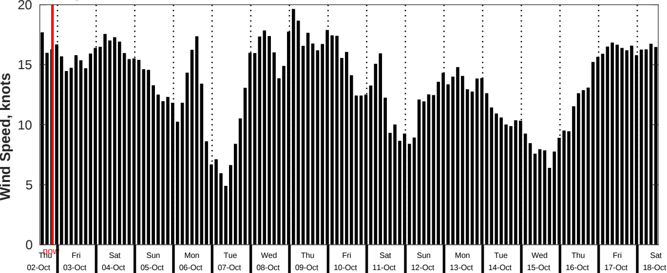
GFS Wind Speed Forecast for NDBC 51209 from 02-Oct-2025 13:00:00 to 18-Oct-2025 13:00:00
